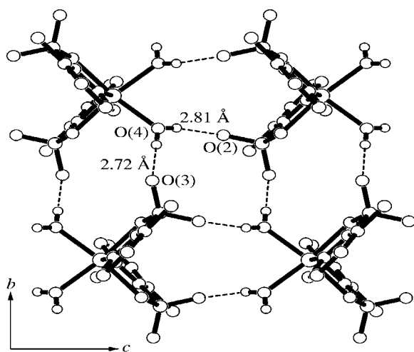
Figure 7. H bonded network of [\text{Mn}(3\text{-mpSO}_3)_2(\text{H}_2\text{O})_2] ( 3 ) parallel to the bc plane
