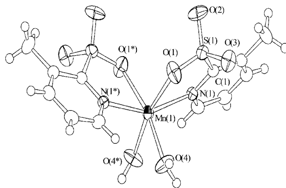
Figure 3. ORTEP drawing of [Mn(3-mpSO 3 ) 2 (H 2 O) 2 ] (3) showing the numbering scheme
