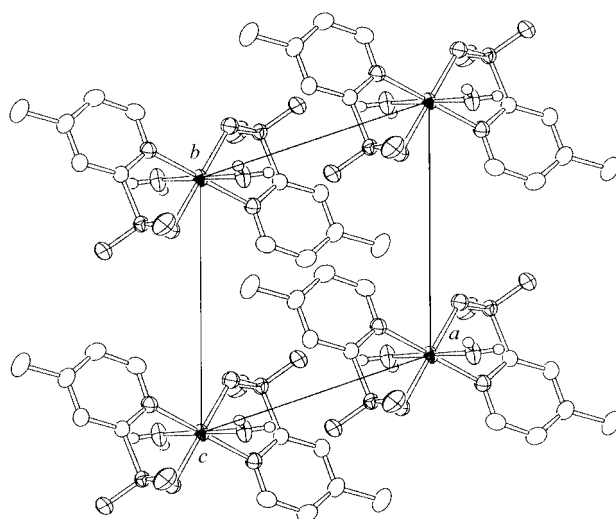
Figure 13. Crystal packing of [\text{Co}(\text{4-mpSO}_3)_2(\text{H}_2\text{O})_2] ( 9 ) when viewed along the c axis
