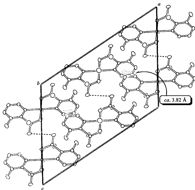
Figure 15. Crystal packing of [\text{Ni}(\text{3-mpSO}_3)_2(\text{H}_2\text{O})_2] \cdot \text{H}_2\text{O} ( 10 ) when viewed along the b axis
