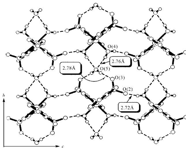
Figure 14. H-bonded network of [\text{Ni}(\text{3-mpSO}_3)_2(\text{H}_2\text{O})_2] \cdot \text{H}_2\text{O} ( 10 ) parallel to the bc plane
