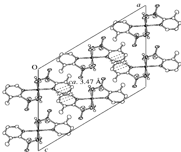
Figure 8. Crystal packing of [\text{Mn}(3\text{-mpSO}_3)_2(\text{H}_2\text{O})_2] ( 3 ) when viewed along the b axis
