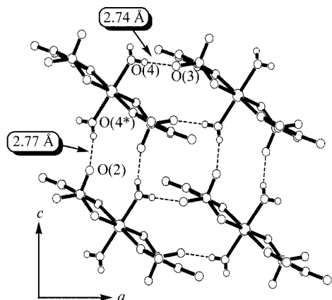
Figure 12. H-bonded network of [\text{Co}(\text{4-mpSO}_3)_2(\text{H}_2\text{O})_2] ( 9 ) parallel to the ac plane
