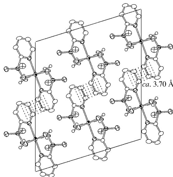
Figure 10. Crystal packing of [\text{Zn}(\text{PySO}_3)_2(\text{H}_2\text{O})_2] ( 8 ) when viewed along the b axis
